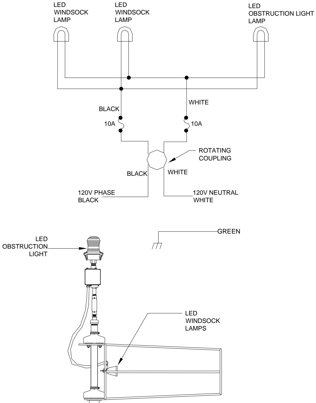
Figure 30. 120 VAC 36" Internal LED Light
