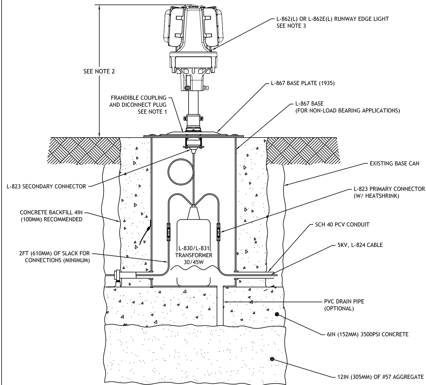
EXAMPLE OF BASE MOUNTED L-862(L)/L-862E(L) FIXTURE INSTALLATION IN EXISTING SHOULDER SECTION
