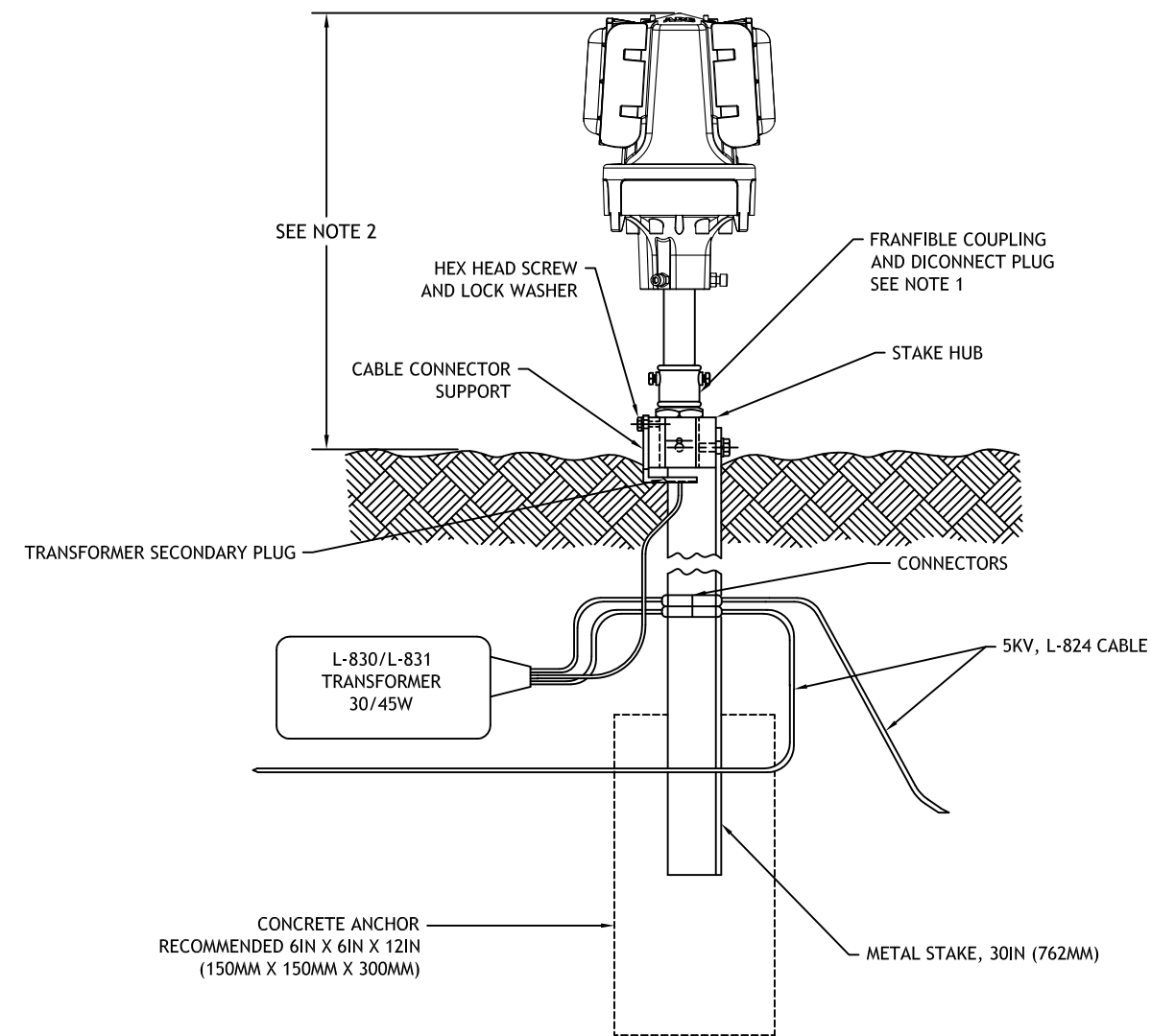
EXAMPLE OF STAKE MOUNTED L-862(L)/L-862E(L) FIXTURE INSTALLATION
