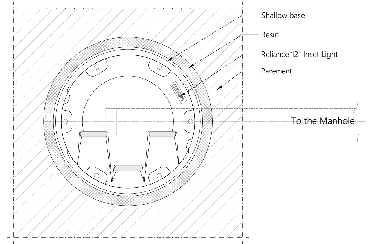
TOP VIEW RELIANCE 12" INSET UNIDIRECTIONAL 3 windows Scale 1/5
