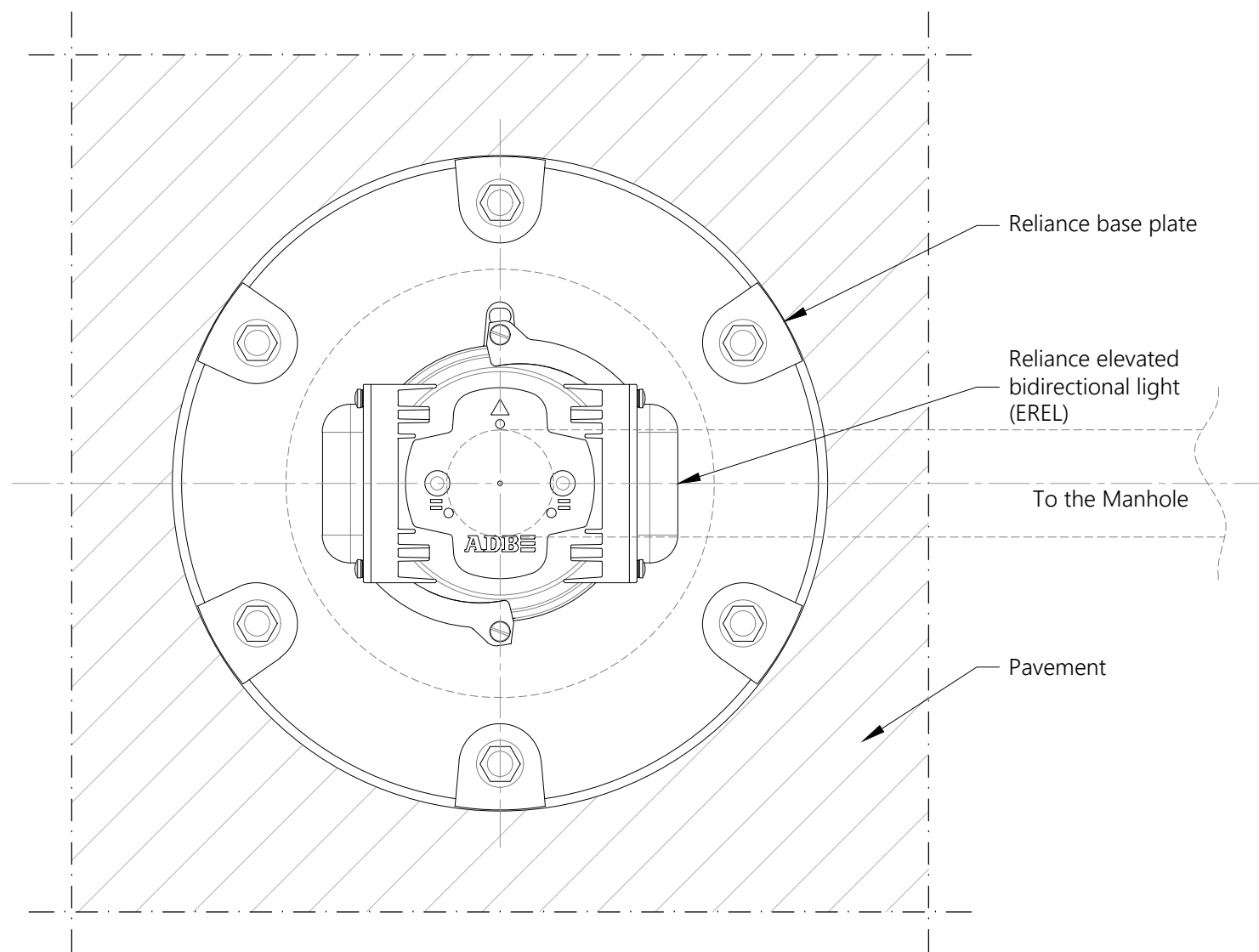
○ TOP VIEW RELIANCE BIDIRECTIONAL ELEVATED LIGHT Scale 1/3
