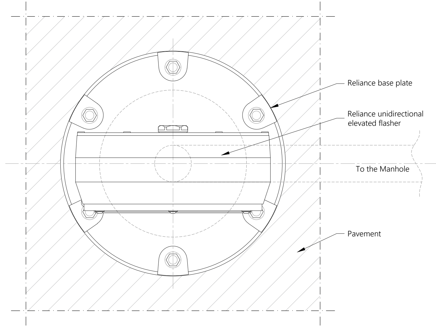
TOP VIEW RELIANCE UNIDIRECTIONAL ELEVATED FLASHER Scale 1/3
