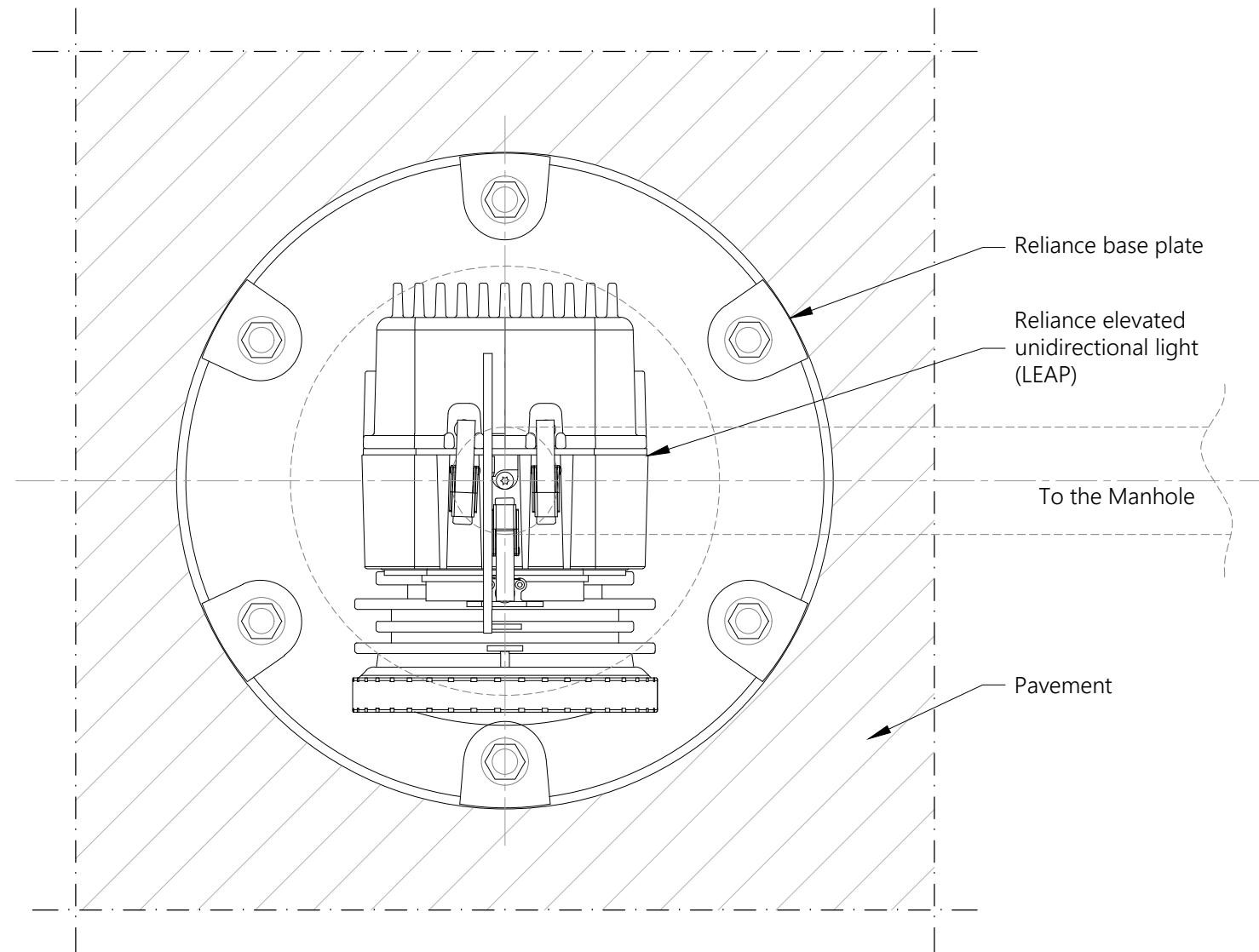
TOP VIEW RELIANCE UNIDIRECTIONAL ELEVATED LIGHT Scale 1/3
